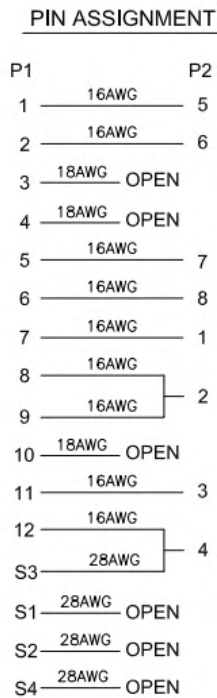
Figure 8. CPU 8-Pin to PCIe 16-Pin Power Adapter Pin Assignments
