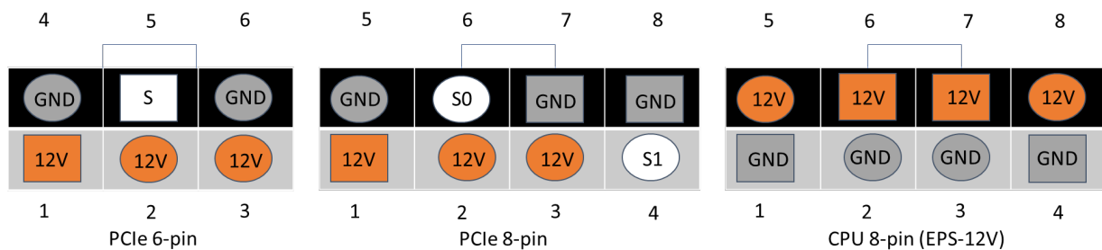
Figure 2. Power Connectors
