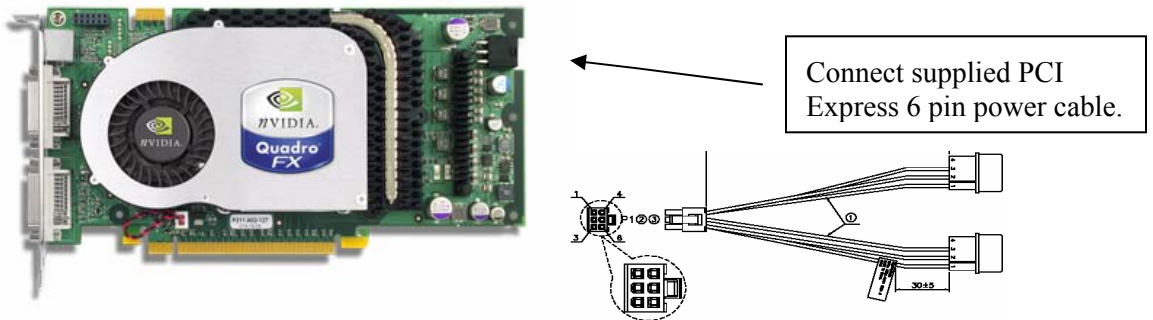
Figure 1: PCI Express power configurations for use of the NVIDIA Quadro FX 3400 by PNY (Using PCI Express 6 pin Power Cable).
